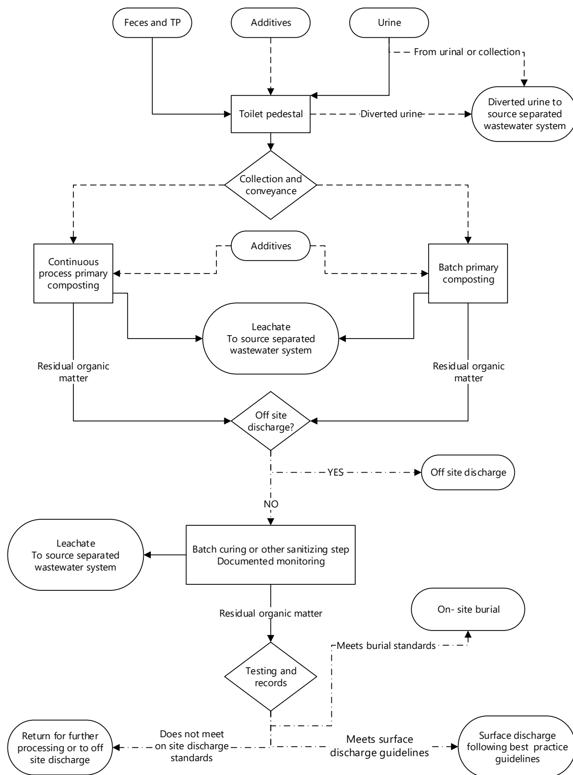
Figure A- 2. Composting toilet flow path
